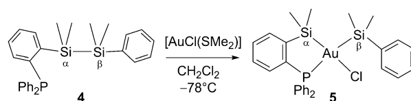
Scheme 3. Synthesis of complex 5 by oxidative addition of the \sigma -Si-Si bond of the monophosphine-disilane 4 at gold.
