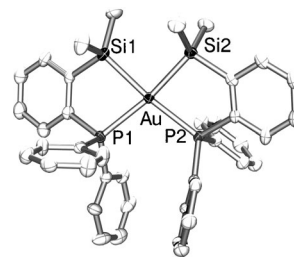
Figure 1. View of complex 3 in the solid state (ellipsoids set at 50% probability; hydrogen atoms, counteranion, and solvate molecules omitted for clarity). Selected bond lengths [Å] and angles [°]: Au–P1 2.4135(6), Au–P2 2.4176(6), Au–Si1 2.4128(6), Au–Si2 2.4213(6); P1–Au–P2 103.63(2), Si1–Au–Si2 89.95(2), P1–Au–Si1 84.67(2), P2–Au–Si2 82.16(2).
