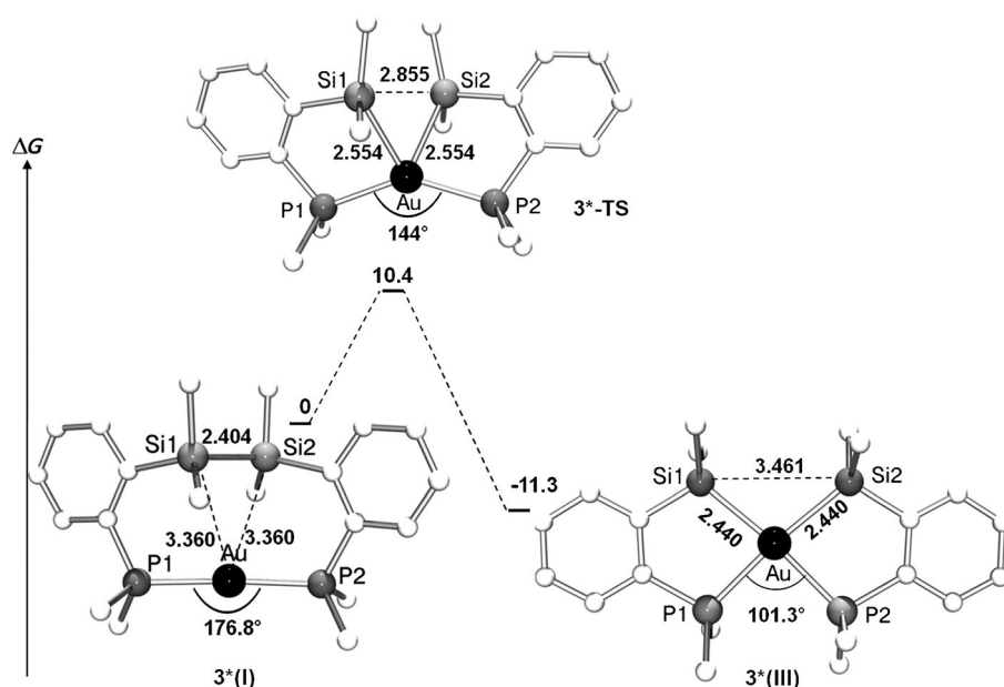
Figure 2. Energy profile computed at the B3PW91/SDD + f(Au),6-31G** (Si,P,C,H) level for the oxidative addition of the \sigma -Si-Si bond in complex 3* . Free energy \Delta G at 25 °C including ZPE correction [kcal mol -1 ], interatomic distances [Å], angles [°].
