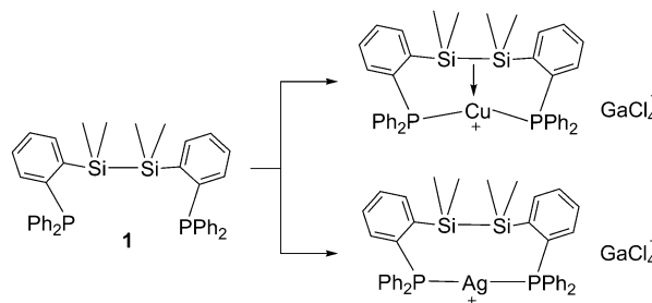
Scheme 1. Coordination of the diphosphine–disilane 1 to copper and silver.
