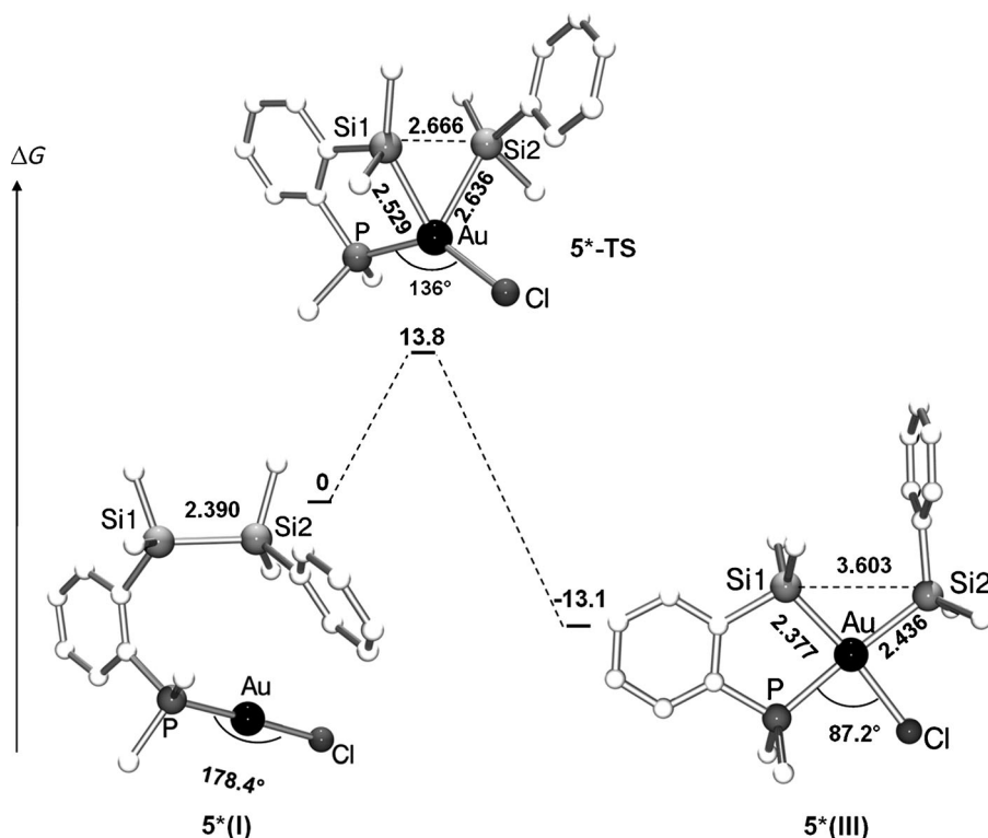
Figure 3. Energy profile computed at the B3PW91/SDD + f(Au),6-31G** (Si,P,C,H) level for the oxidative addition of the \sigma -Si-Si bond in complex 5* . Free energy \Delta G at 25 °C including ZPE correction [kcal mol -1 ], interatomic distances [Å], angles [°].
