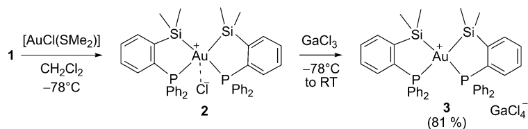
Scheme 2. Synthesis of complexes 2 and 3 by oxidative addition of the \sigma -Si–Si bond of the diphosphine–disilane 1 at gold.
